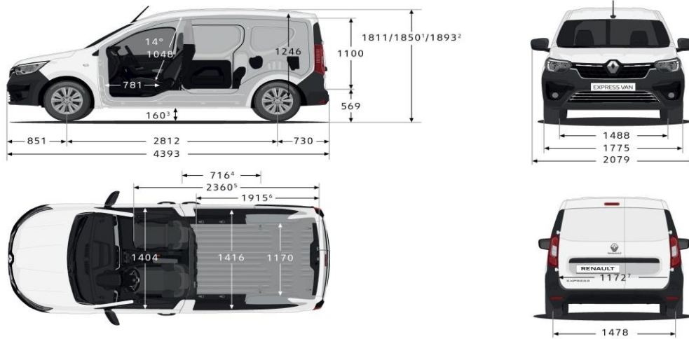
Dimensions (mm)
