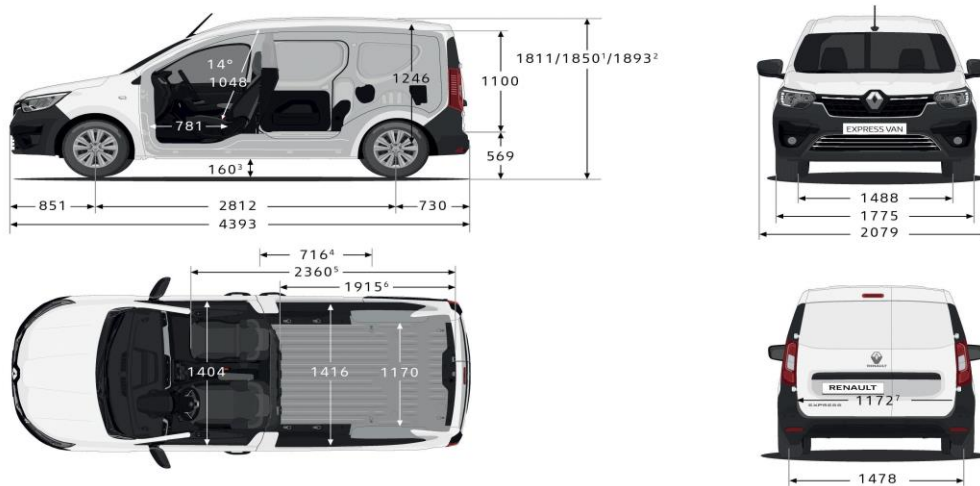
Dimensions (mm)
