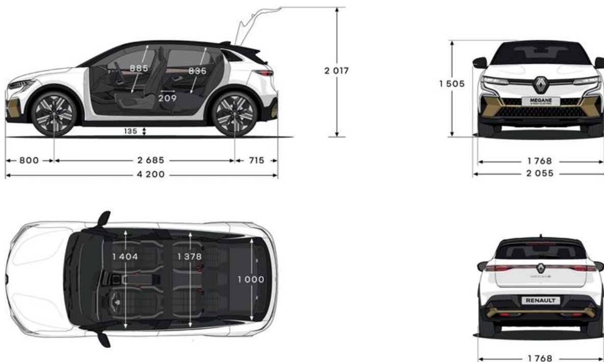
Dimensions (mm)
