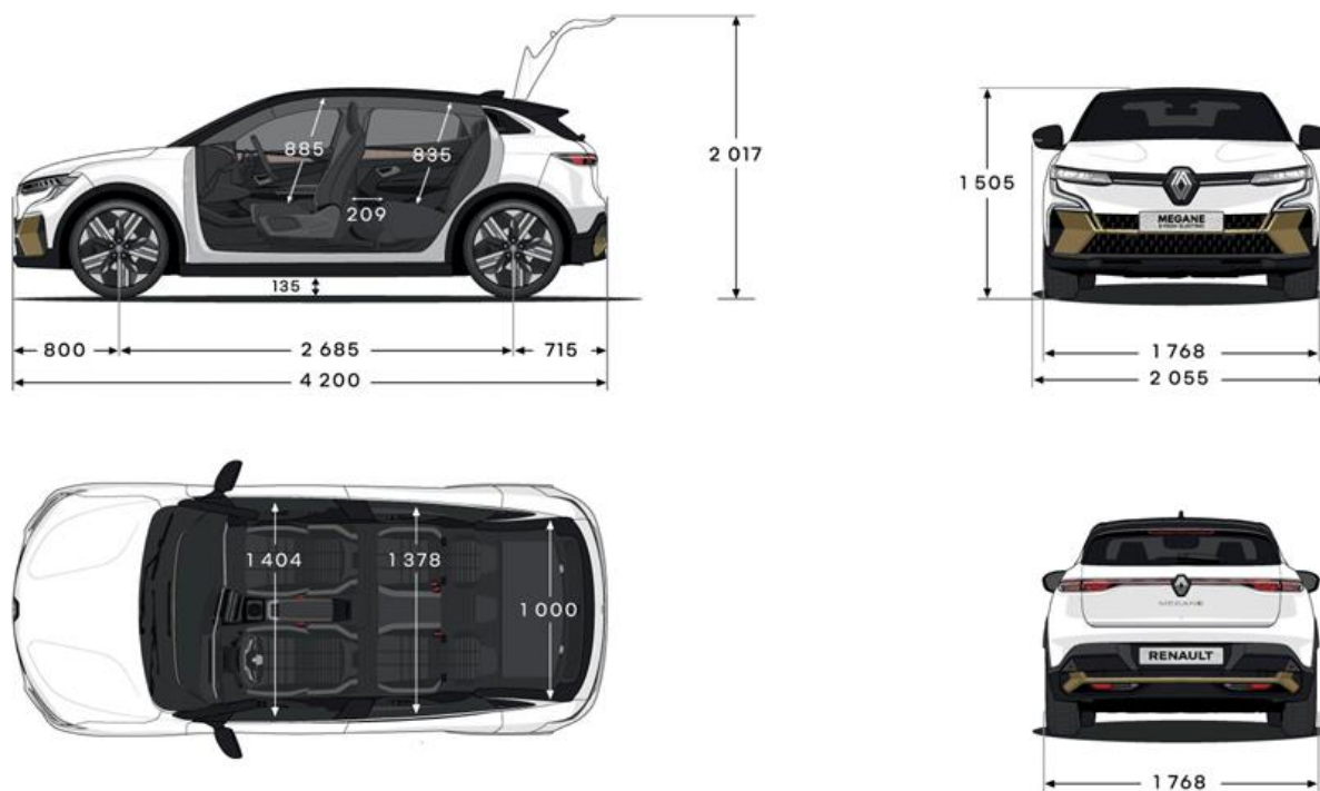
Dimensions (mm)
