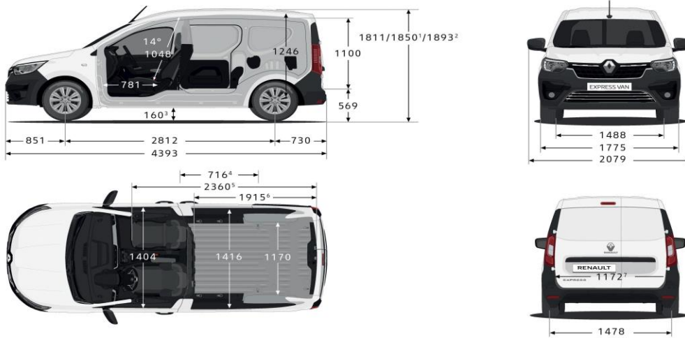
Dimensions (mm)
